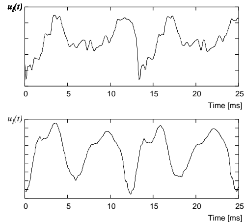
Figure 3: Laryngeal airflow of kargyraa voice obtained by inverse-filtering. Top: Singer A. Bottom: Singer B.
