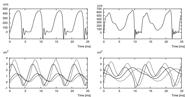
Figure 5: Synthesized laryngeal flows using the 2 \times 2 -mass model. Left: Simulated drone voice. Right: Simulated double-periodic kargyraa voice. Laryngeal flow (top) and the vocal and ventricular fold vibrations (bottom).
